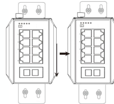
Schematic diagram of wall mounted installation of industrial machine
