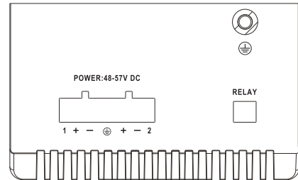
Figure 3-2 AIS2003P side panel
