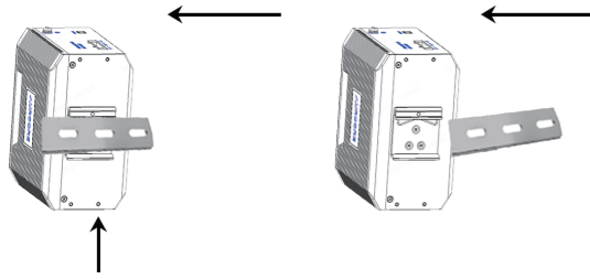
Figure 4-1 Schematic diagram of industrial machine guide rail installation
